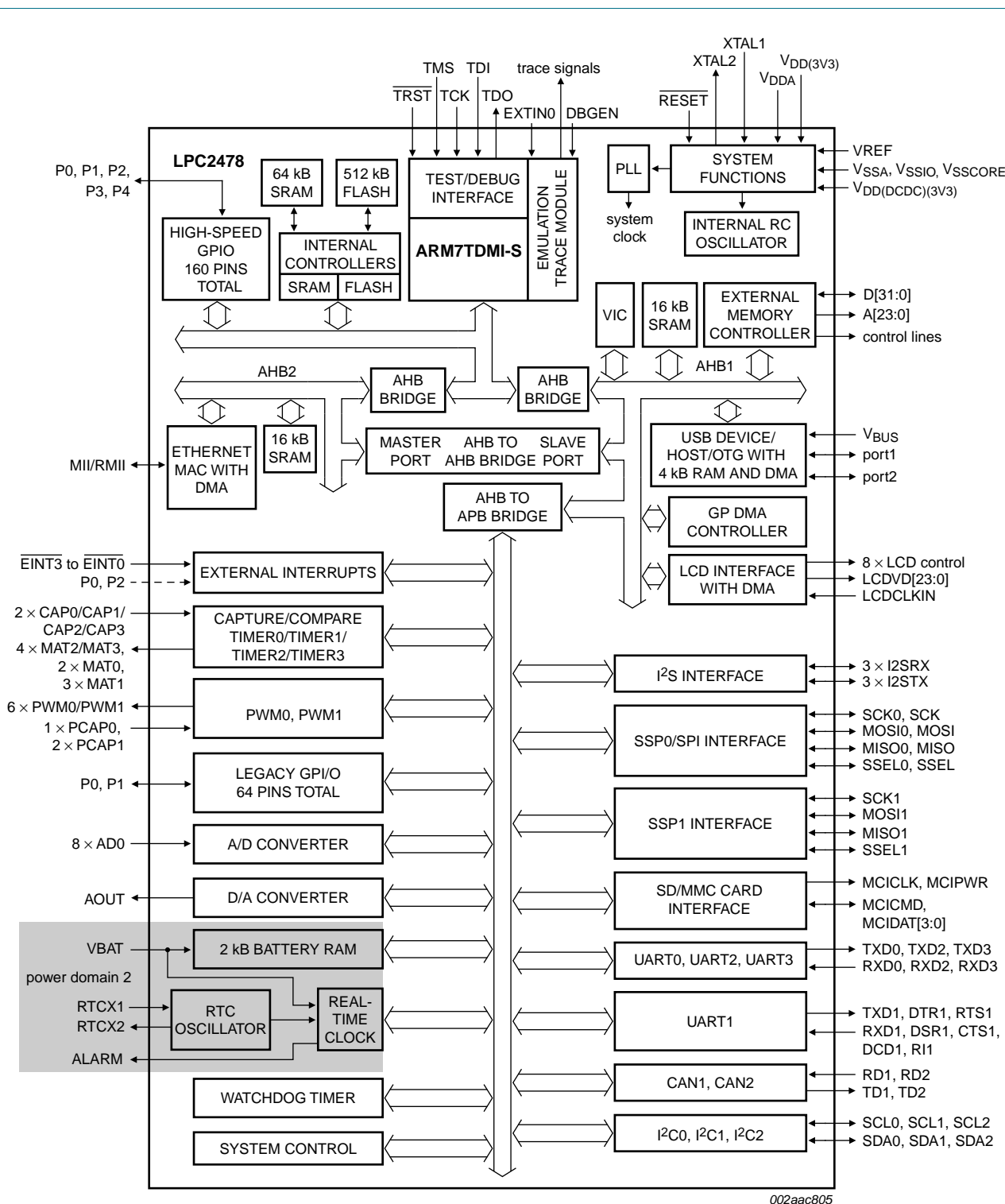
Fig 1. LPC2478 block diagram
